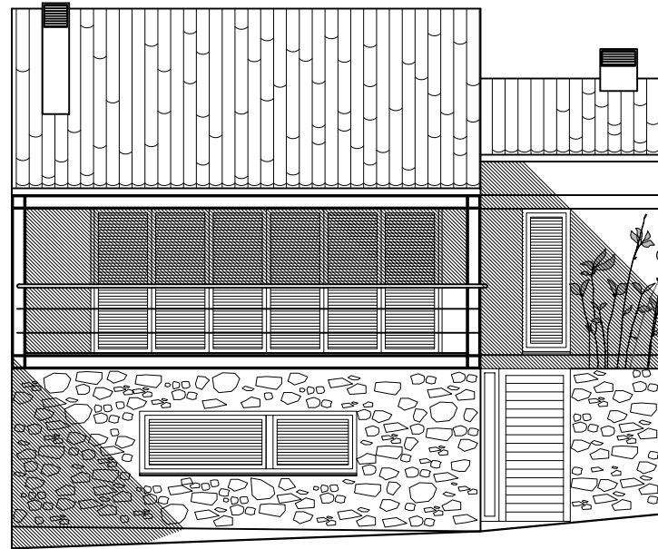
ALZADO PRINCIPAL
